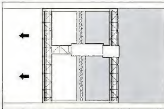
Auger midway between rollers distributes asphalt
